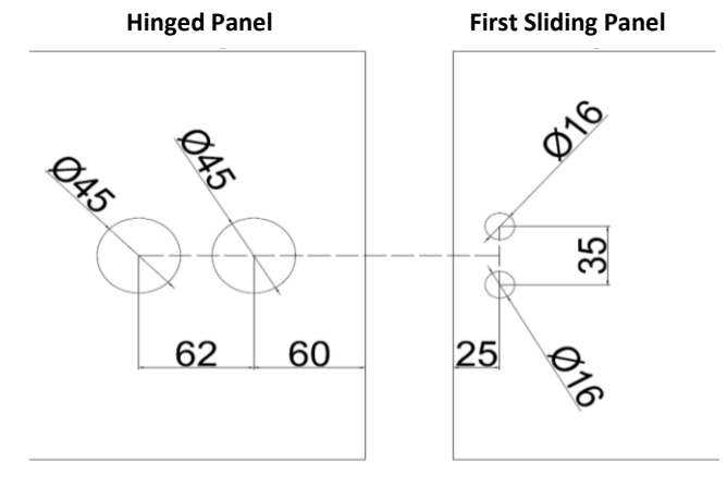
GLASS TO GLASS LOCK GLASS HOLE DETAIL
