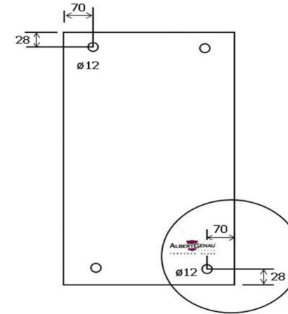
GLASS DETAIL WITH HOLE
