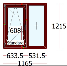
UșăBalcon20 - 1 buc.
