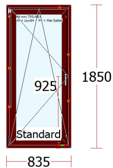
UșăBalcon16 - 1 buc.
