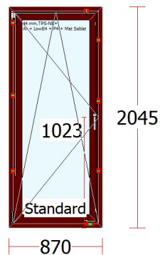
UșăBalcon20 - 1 buc.
