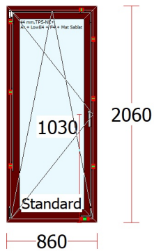
UșăBalcon21 - 1 buc.
