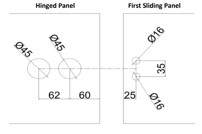
GLASS TO GLASS LOCK GLASS HOLE DETAIL
